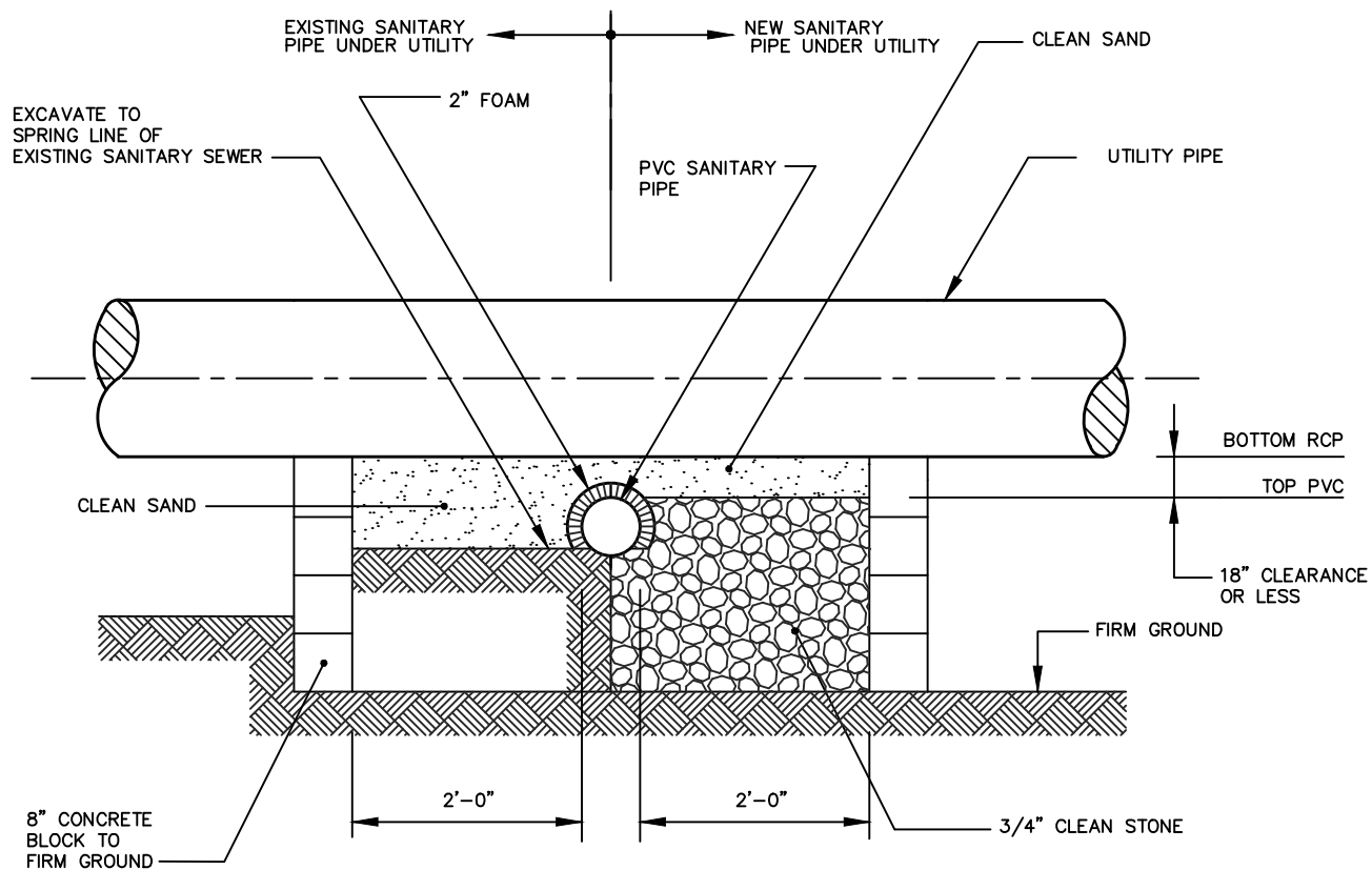
SANITARY SEWER – UTILITY CROSSING DETAIL NOT TO SCALE
