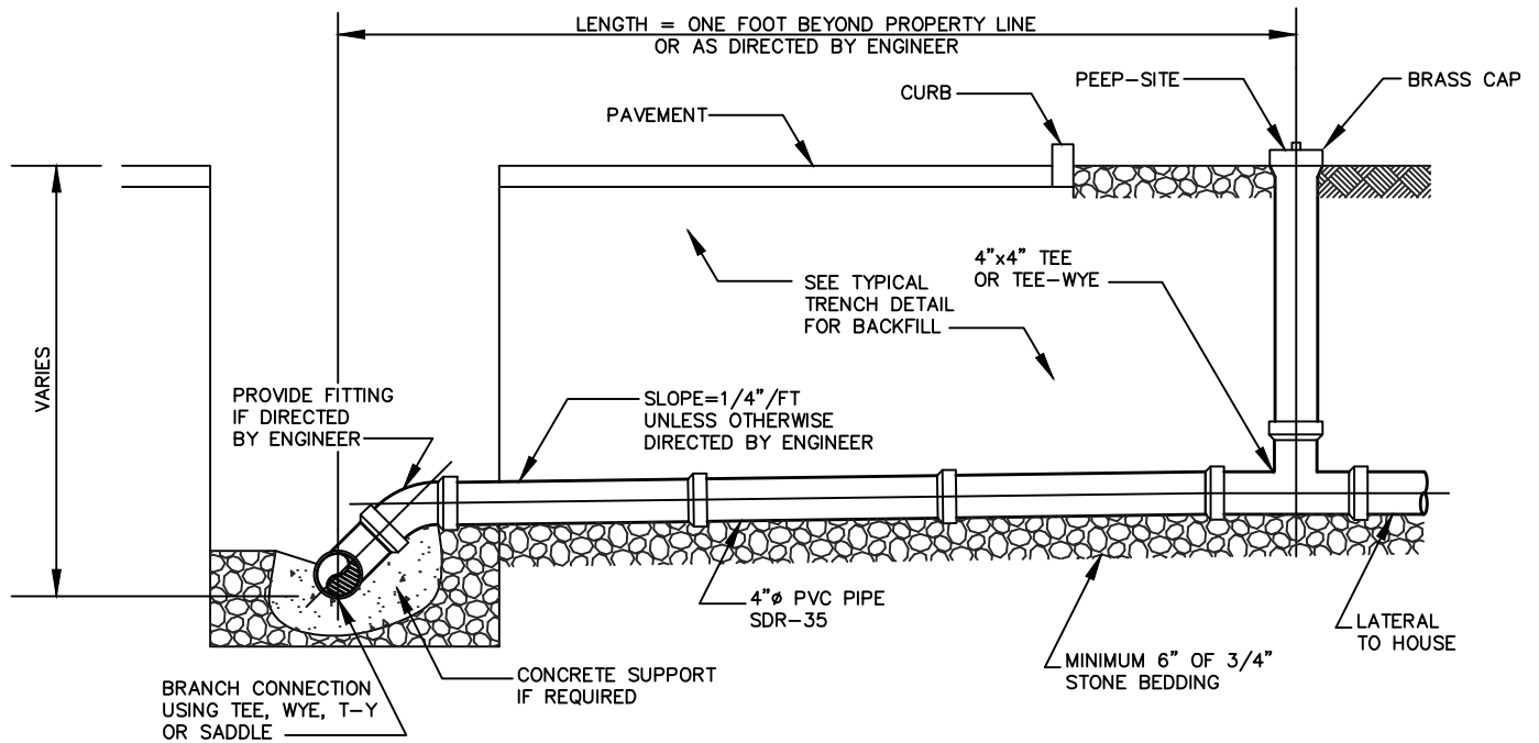
TYPICAL HOUSE CONNECTION NOT TO SCALE
