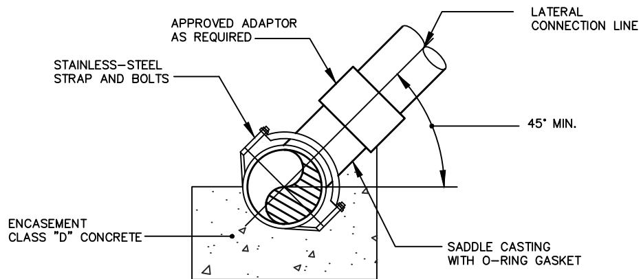
LATERAL DETAIL CONNECTION BY SADDLE TAP TO PIPE NOT TO SCALE
