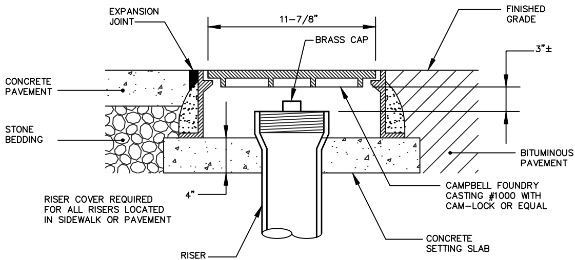
CLEANOUT RISER COVER DETAIL NOT TO SCALE
