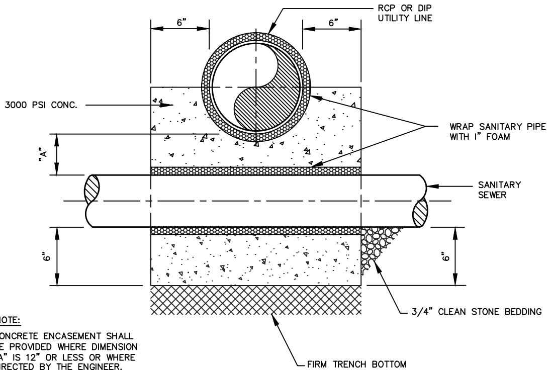
PIPE CROSSING DETAIL NOT TO SCALE
